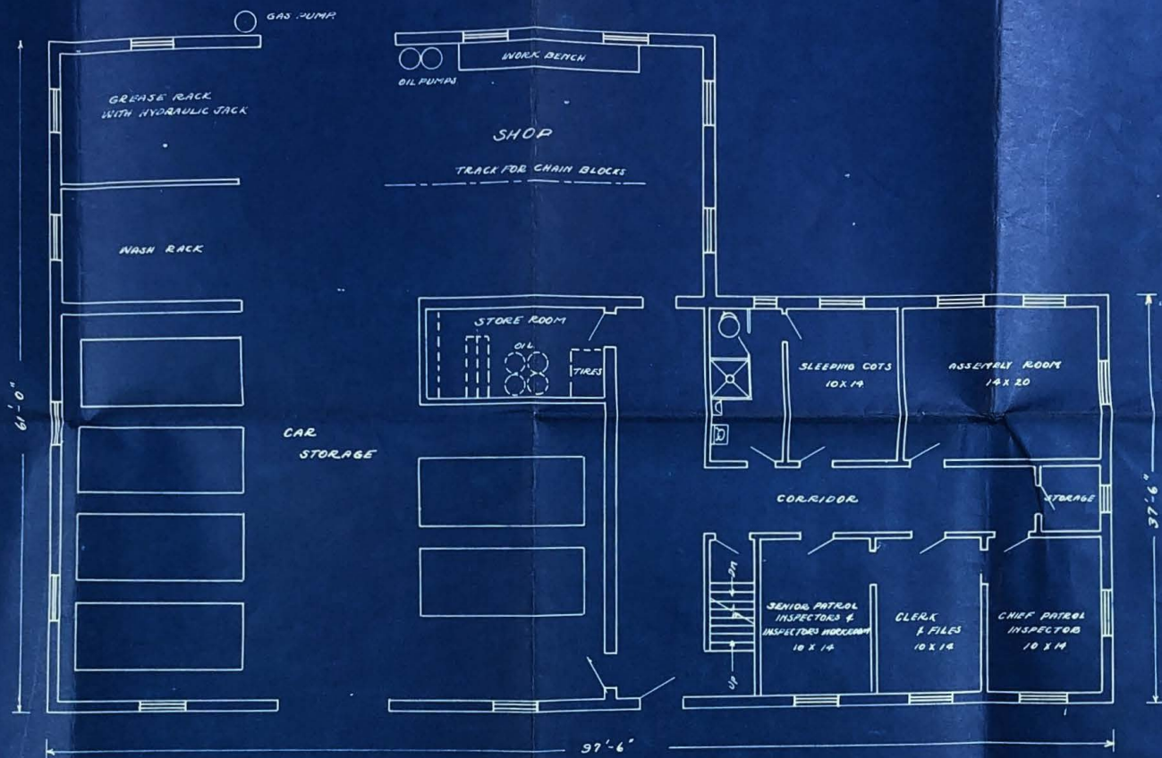
FIRST FLOOR PLAN SCALE - \frac{1}{16}'' = 1'
